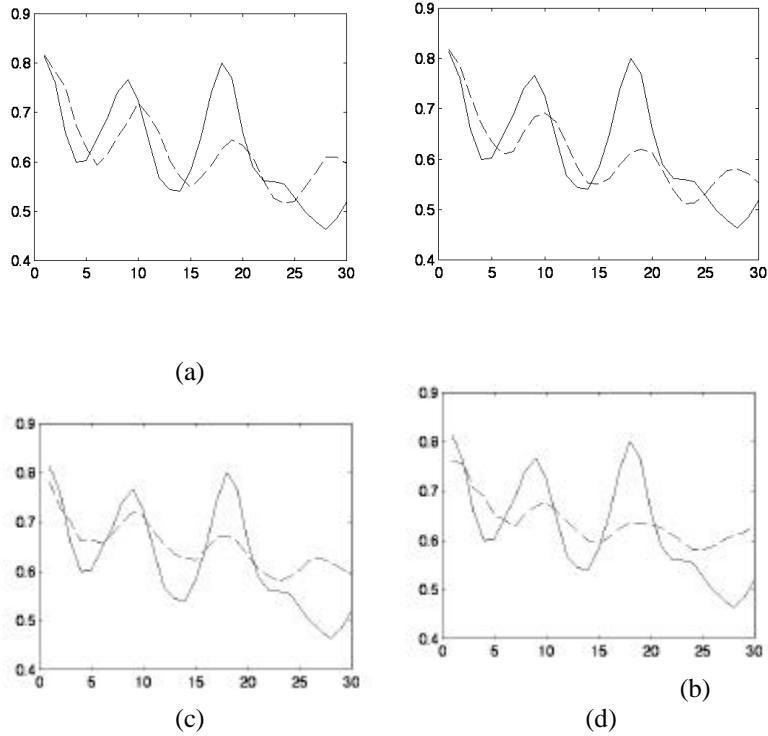
Fig.2: (a) 100 clusters in the input space and 5 in the deformations spaces (b) 200 clusters in the input space and 3 in the deformations spaces (c) 200 clusters in the input space and 5 in the deformations spaces (d) 250 clusters in the input space and 4 in the deformations spaces.
